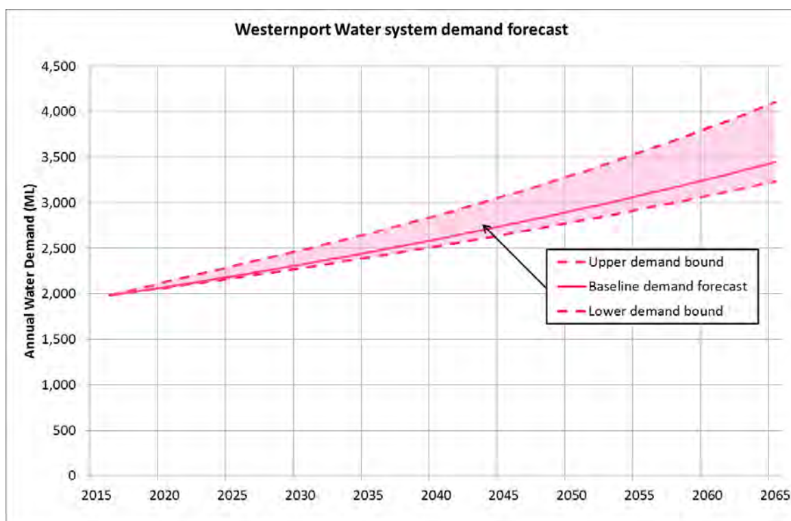
Figure 4 Westernport Water 2017 UWS demand forecast
